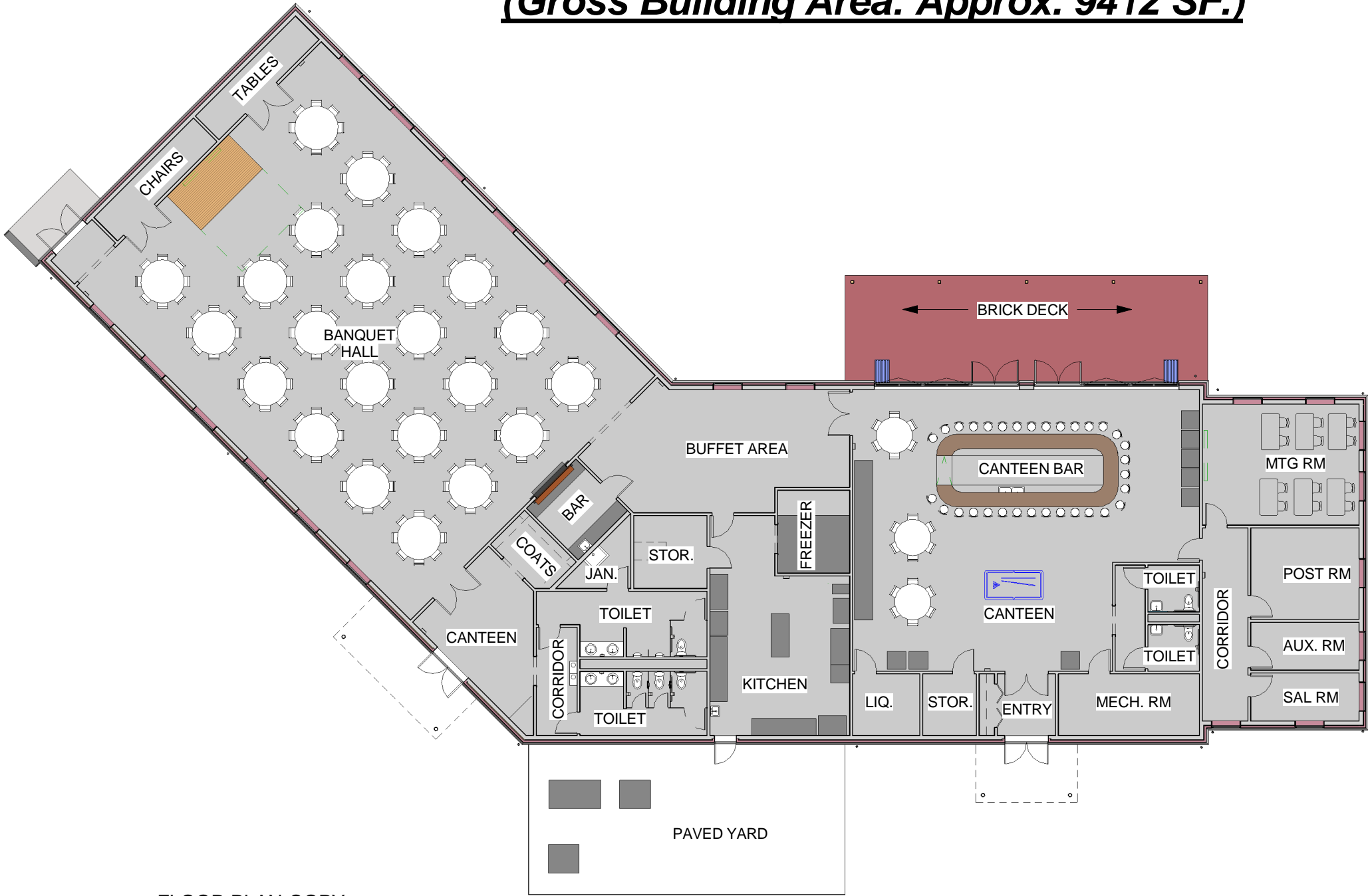
① FLOOR PLAN-COPY 1/16" = 1'-0"
